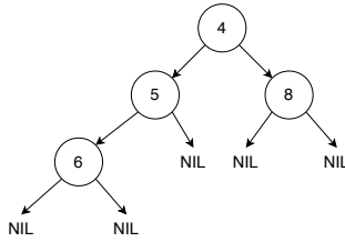
图 8.6: rank(4) = 2, rank(6) = rank(8) = rank(5) = 1
