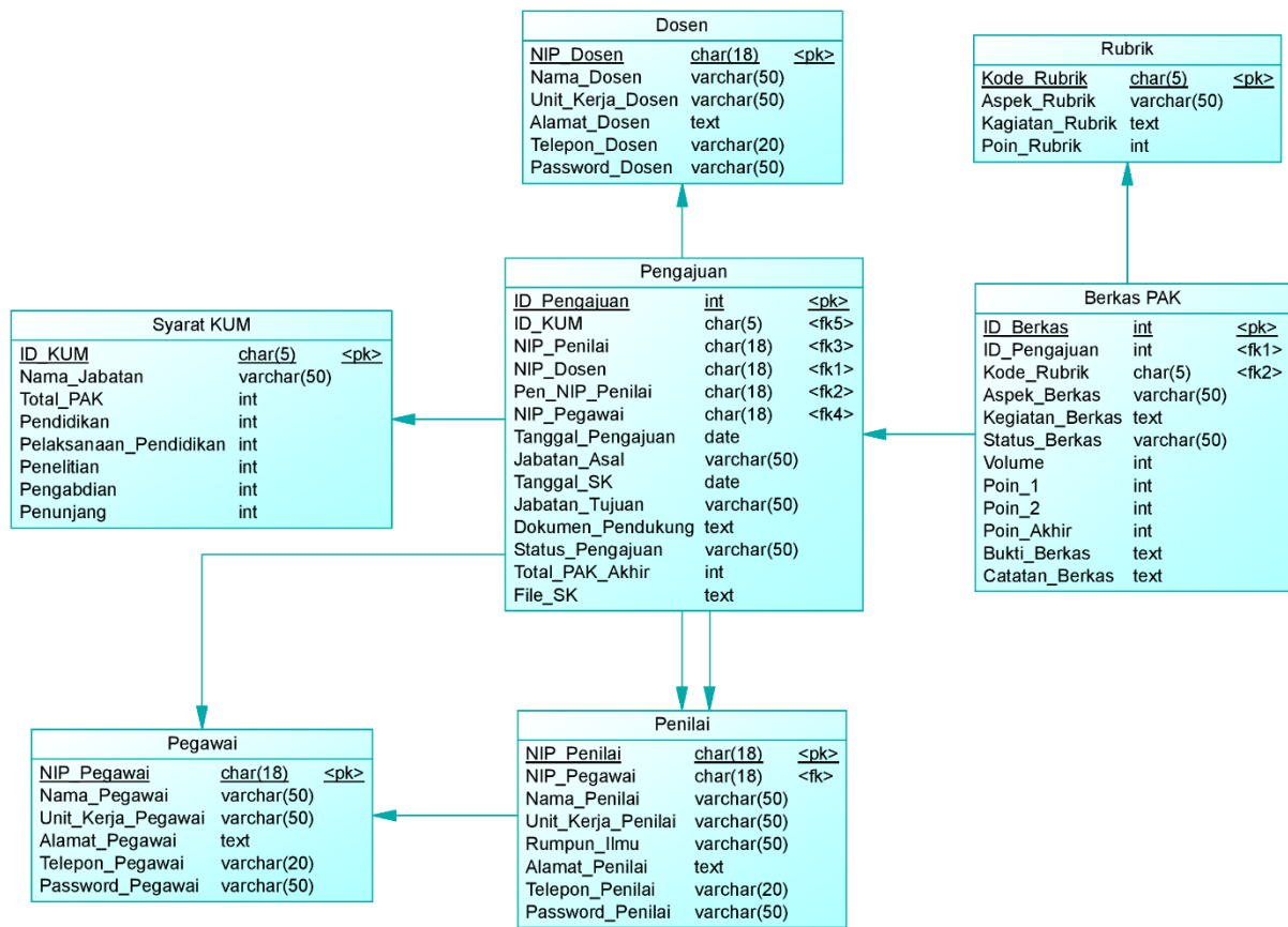
Gambar 29. Physical Data Model
