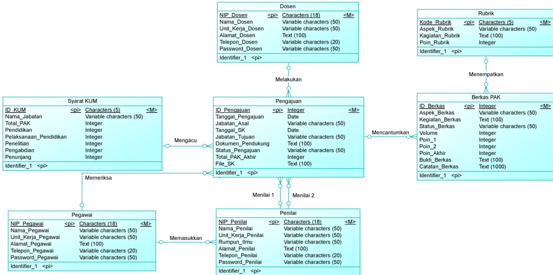
Gambar 28. Conceptual Data Mode
