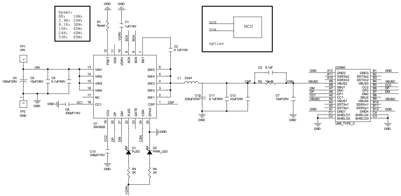
Type-C Port Output Application
