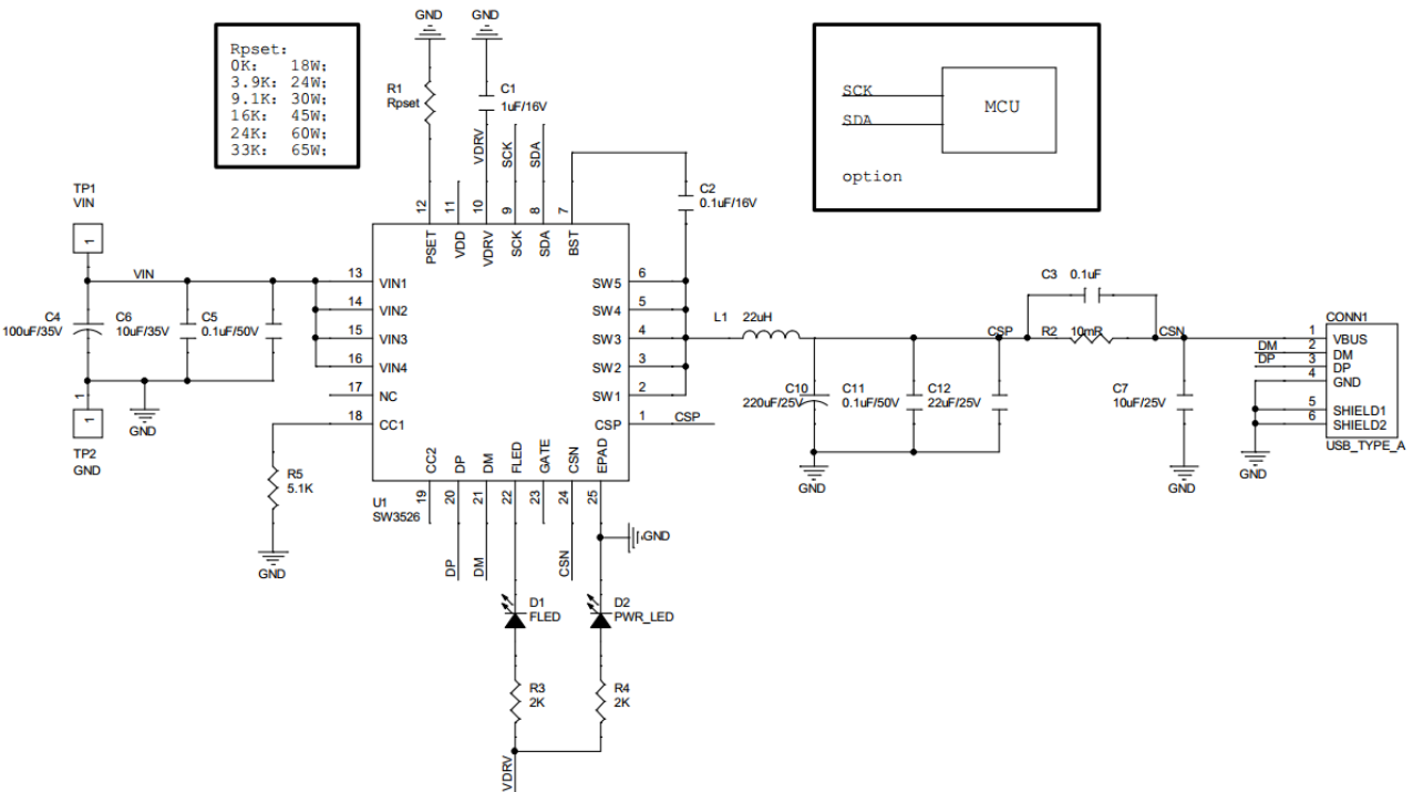
Type-A Port Output Application
