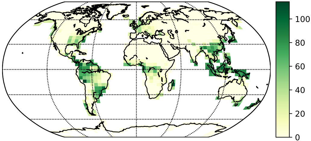
FATES_VEGC [Mg/ha]
